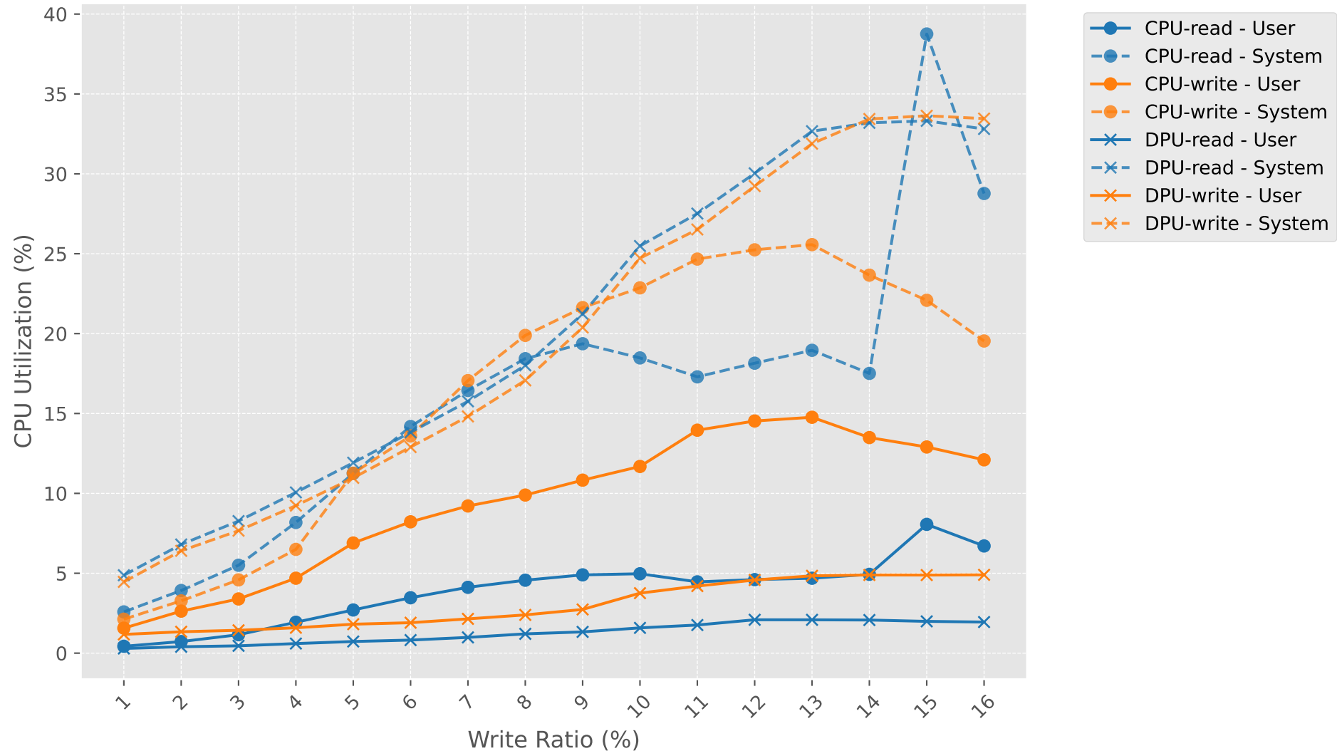
CPU Utilization vs Write Ratio (nbcpu-bw)
